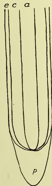
FIG. 4.—Diagram of longitudinal section of young root. a, axial cylinder; c, cortex; e, epidermis; p, root cap.
