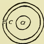
FIG. 5.—Cross section of young root.
