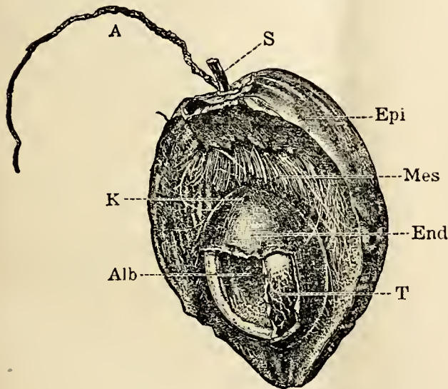
FIG. 3. STRUCTURE OF THE COCOA-NUT. \times \frac{1}{3}
