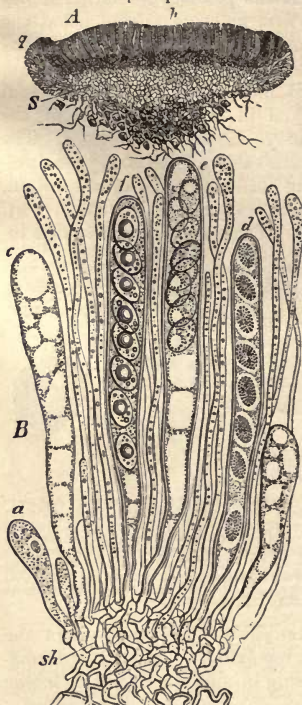
Fig. 32.— Peziza convexula . A , vertical section of the whole plant; h , hymenium—i.e., the layer in which the spore-forming sacs lie, S , the tissue of the fungus enveloping the hymenium at its edge q in a cup like manner; at the base of the tissue S fine threads arise, which grow between the particles of earth. B , a small portion of the hymenium; sh , sub-hymenial layer of densely interwoven filaments (hyphae); a to f , spore-forming sacs (asci), with thin filaments (paraphyses) between them. A \times 20, B \times 550.—After Sachs.
