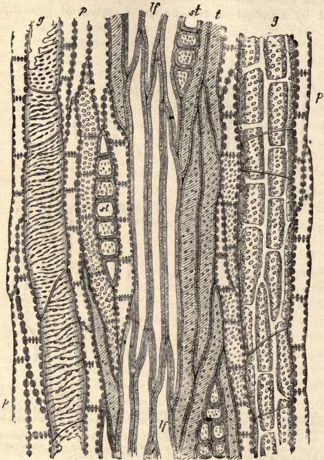
Fig. 328.—Tangential section of the stem of Allanthus glandulosa , through the secondary xylem: g, g , pitted vessels; p, p , xylem parenchyma; st, st , medullary rays in cross section; f, f , fibrous tissue (wood cells); t , tracheides. Highly magnified.—After Sachs.
