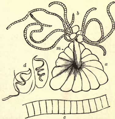
Fig. 229.— Chara fragilis . a, an isolated shield, m, seen from within, with manubrium bearing the filaments, b, in which the spermatozoids are developed; c, a small portion of one of the filaments, the spermatozoids not shown; d, two free spermatozoids. a and b \times 50 ; c and d \times 300 .—After Thuret.
