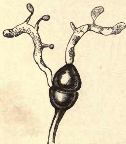
Fig. 218.—Germinating teleutospore of Puccinia Molinia , showing promycelium and sporidia.—After Tulasne.
