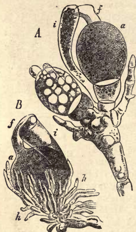
Fig. 194.—Sexual organs of Peziza confluens , highly magnified. A, at time of fertilization; a, carpogonium; f, trichogyne; i, anthridium. B, after fertilization; h, h, the hyphae from which the receptacle is developed.—After Tulasne.
