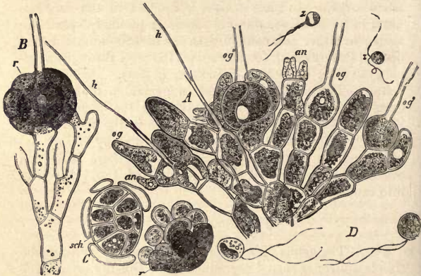
Fig. 183. — Coleochaete pulvinata . A , portion of fertile plant; an , antheridia; og , carpogonia—each with a trichogyne; z, z , spermatozooids; h , halra, with sheathing bases. B , fertilized carpogonium surrounded by covering, r ("pericarp"), the whole constituting the sporocarp. C , sporocarp burst open, showing the interior tissue, sch ; r , cortical cover ("pericarp"). D , zoospores (swarm-spores) from C . \times 350 .—After Pringsheim.
