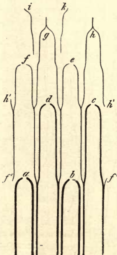
Fig. 317.—Diagram showing the arrangement of the fibro-vascular bundles in Stachys angustifolius . a, b, d, c, f, e, g, h, i, k , the points from which the successive pairs of leaves spring.—After Nägeli.
