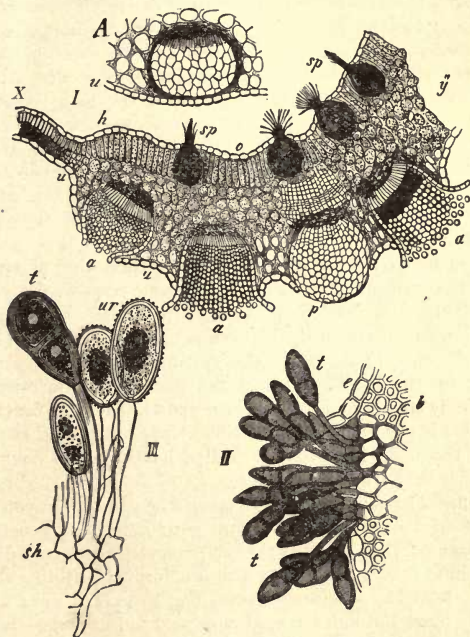
Fig. 216.—Several stages of Puccinia graminis . A, part of a vertical section of a leaf of the Barberry ( Berberis vulgaris ), with a young unopened æcidium fruit; u, epidermis. I, section of a Barberry leaf, natural thickness at X, greatly thickened from h toward y; u, epidermis of the under surface; o, of the upper surface; p, unopened æcidium fruit; a, a, a, opened æcidium fruits; sp, sp, spermagonia. II, a mass of teleutospores on a leaf of Couch-grass ( Triticum repens ); e, the ruptured epidermis; b, sub-epidermal fibres of the grass leaf. III, three uredospores, ur, with one teleutospore, t; sh, sub-hymenial hyphæ. All highly magnified.—A and I. after Sachs; II. and III. after De Bary.
