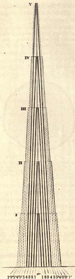
FIG. 830.—An ideal vertical section of a dicotyledonous stem, five years old. I., II., III., IV., V., the successive heights attained in its annual growth; m, pith; 1, 2, 3, 4, 5, the annual xylem layers corresponding respectively to the annual phloem layers, 1', 2', 3', 4', 5'.—After Duchartre.
