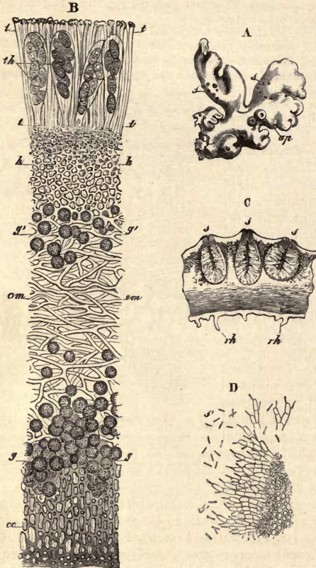
Fig. 202.— Parmelia aipollia . A, a portion of a thallus with two apothecia, ap , and several spermagonia, s, s . B, transverse section of thallus through an apothecium; cc , cortical layer of pseudo-parenchyma; g, g' , gonidial layers; cm , medullary layer; h, h , hypothecium; t, t, t , the hymenium; th , asci (thecae), with ascospores. C, section through three spermagonia, s, s, s ; rh, rh , rhizoids. D, sterigmata from the interior of a spermagonium, bearing spermatia, s', s' .—After Tulasne.
