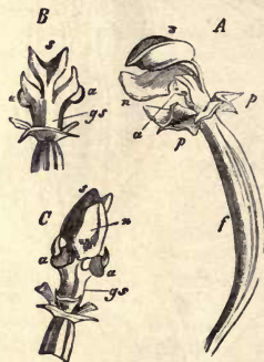
Fig. 362 — Sexual organs of the flower of Cypripedium calceolus , the perianth, p , removed. A , side view. B , back view. C , front view. f , the inferior ovary; gs , the column or gynostemium; aa , stamens; s , sterile stamen or staminode; n , stigma.— After Sachs.
