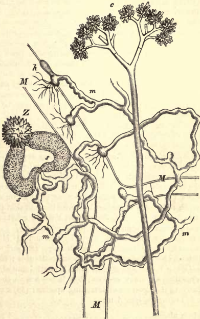
Fig. 162.— Piptocephalis Fresentiana , parasitic upon the hyphæ, M, M, M , of Mucor Mucedo . m, m , parasitic hyphæ, attached to their host by the haustoria, h ; c , conidial spores ; s, s , the two branches which conjugate and form the zygospore, Z . Highly magnified.—After Brefeld.
