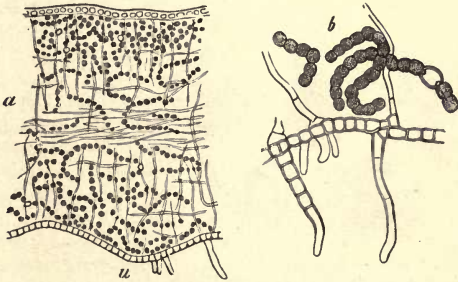
Fig. 210.— Mallotium (or Leptogium ) Hildenbrandii . 'a, vertical section through the thallus, u, the under side, \times 190 ; b, portion of a very thin section near the under side, showing three gonidia chains, two hyphæ, a portion of the lower liminary tissue, and two large and several small hairs, which are organs of attachment, \times 390 .—After De Bary.
