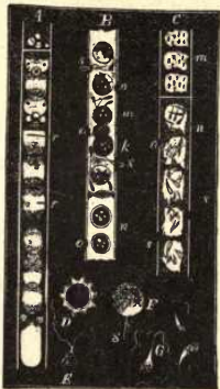
Fig. 165.— Sphæroplea annulina . A , ordinary filament; r , chlorophyll masses. B , filament consisting of oogonia, the contents breaking up into oospheres; o, o , openings for entrance of spermatozooids; s, s , spermatozooids entering the oogonia; m and k , oospheres at the instant of fertilization; n , fertilized oospheres, now enclosed in a thin cell-wall. C , filament consisting of antheridia; s, s , the escaping spermatozooids, issuing through the openings o o . D , an oospore with its thick coats of cellulose. E , zoospore (vegetative zoogonidium). F , oosphere in the act of being fertilized by a spermatozoid, s . G , spermatozooids.—After CErsted.
