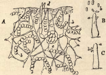
Fig. 207.—Sexual organs of Collema microphyllum . A , section of thallus; a, a , hyphæ; b, b , the Nostoc-like gonidia; c , ascogonium; d , the exerted trichogyne. B , the spermata, b , surrounding the exerted trichogyne, a . C , coalescence of a spermatium, b , with trichogyne, a . All the figures magnified, B and C much more than A .—After Stahl.
