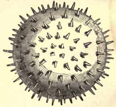
Fig. 11.—Pollen grain of Lavatera trimestris , covered with prickles. \times 200 .—After Duchartre.
