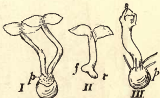
Fig. 271.—I., two young plants of Selaginella Martensii growing from the same spore; at the top of the spore may be seen the projecting prothallium, p . II., a young plant drawn out of the spore, showing the foot, f , on the left below, and the young root, r , on the right. III., a young plant whose first leaves (cotyledons) have been removed, leaving only their stipules, s ; between the latter is seen the dichotomously dividing punctum vegetationis ; p , the prothallium isolated from the spore. I. \times 5 ; II. \times 3 ; III. \times 30 .—After Hofmeister.
