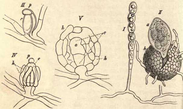
Fig. 188.— I , conidia-bearing hypha of Sphaerotheca pannosa . II , the ripe sporocarp of the same; a , the single ascus escaping from the perithecium, h ; only a few of the hypha-like appendages of the perithecium are shown. III , sexual organs of the same; c , carpogonium; p , antheridium. IV , the formation of the perithecium by the growth of the enveloping cells, h ; c , carpogonium; p , antheridium. V , section of the young sporocarp of Sphaerotheca Castagnei ; c , carpogonium; a , the young ascus; h , h , cells of the perithecium. I and II after Tulasne; III – V after De Bary.
