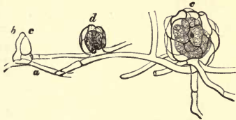
Fig. 189.—The sexual process in Erysiphe Cichoriacearum . a, threads of mycelium; b, auteridium; c, carpogonium; d, young sporocarp; e, older sporocarp. Highly magnified.—After Cæsted.
