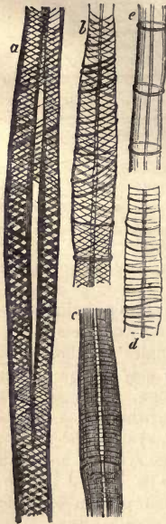
Fig. 24.—Striation of the bast fibres of Ilova carnososa ; a and b , crossed annular striation; c , d , e , varieties of simple annular striation.—After Sachs.
