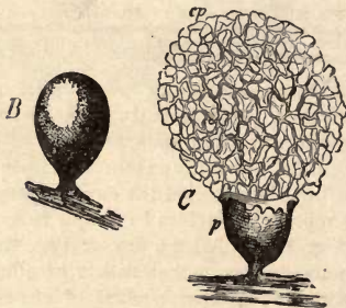
Fig. 144.—Fructification of Arcyria incarnata ( A. adnata of Ritki.). B , young sporangium; C , mature sporangium ruptured; cp , capillitium; p , wall of sporangium. \times 20 .—After Sachs.
