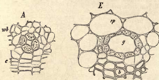
Fig. 115.—Transverse sections of young stem of Ivy ( Hedera helix ). A, young tertiary gum canal, surrounded by four cells; c, cambium; wb, soft bast; E, fully developed canal, g; b, bast; rp, cortical parenchyma. \times 800 .—After Sachs.
