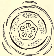
Fig. 520.—Flower diagram of Gordonia Lasianthus .
