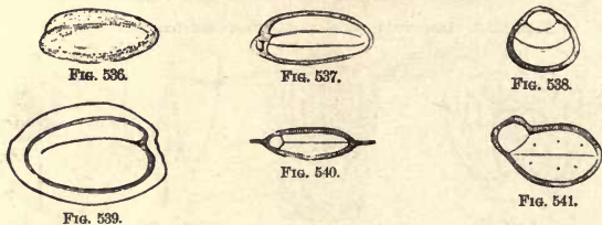
Fig. 536.—Seed of Erysimum . Magnified.
