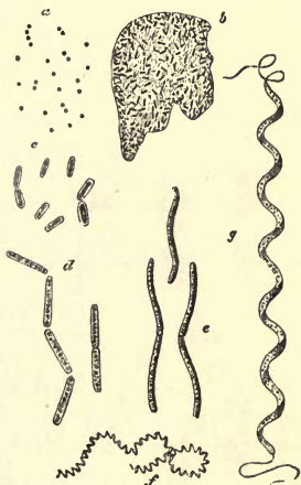
Fig. 145. a, Micrococcus prodigiosus , ( Monas prodigiosus of Ehrenberg); b, Bacterium Termo , zoogloea stage; c, Bacterium lineola ; d, Bacillus ulna ; e, Vibrio Rugula ; f, Spirochæte plicatilis ; g, Spirillum volutans . \times 650 .—After Cohn.
