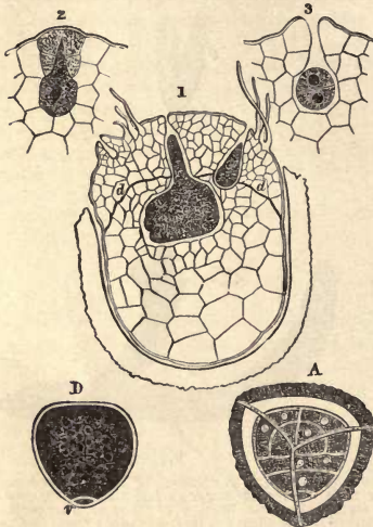
Fig. 276 — Germination of the spores of Selaginella . 1, longitudinal section of a macrospore of S. Martensii ; above the line d is the prothallium, below it the "endospERM"; e, e' , two embryos, the larger one with its suspensor projecting into the neck of the archegonium; at the left of the larger embryo is a young archegonium; several root-hairs are also shown. 2, a young archegonium of the same species, not yet open. 3, an archegonium of the same species, with the germ-cell fertilized and divided into two. A , a microspore of S. caulescens , rendered transparent, showing the division of the contents into the primordial cells; the small lower cell is the rudimentary prothallium. D , later stage of the same, showing the large antheridium filled with sperm-cells; v , the rudimentary prothallium. All magnified.—After Pfeffer.
