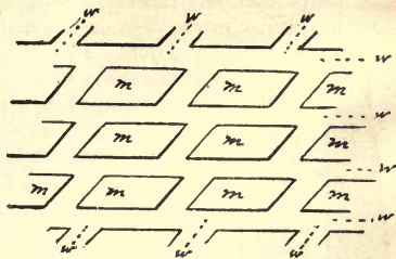
Fig. 22.—Diagrammatic figure to illustrate Nägeli's theory of the molecular structure of the cell-wall; m, m, m , the crystal molecules; w, w, w , the layers of water which separate the molecules. The water layers are represented as very thin; they are frequently much thicker in proportion to the diameters of the molecules. (NOTE.—It must be borne in mind that this figure is purely diagrammatic.)
