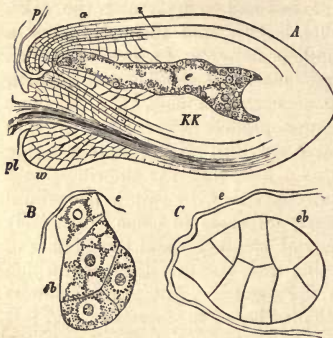
Fig. 307.— A , a longitudinal section of the anatrochous ovule of Viola tricolor , after fertilization. pl , the placenta ; w , the raphé, swollen at this point ; a , the outer coat of the ovule ; i , the inner ; p , the pollen-tube which has entered the micropyle ; e , embryo sac, with the very young embryo at the micropylar end, and numerous free endosperm cells at the other. B , apex of embryo sac, e (much more magnified) ; eb , very young embryo of two cells, supported by a two-celled suspensor. C , the same, further advanced. All the figures highly magnified.—After Sachs.
