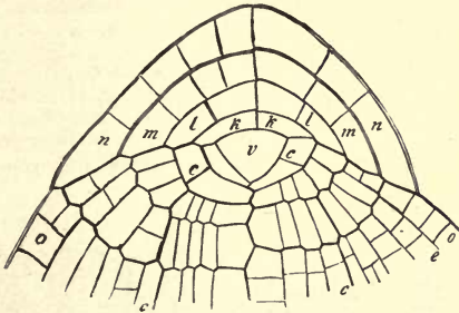
Fig. 257a.—Longitudinal section of the apex of the root of Pteris hastata . v , apical cell; o, o , epidermis; e , cortical tissue; c-c, c-c , the primary fibro-vascular bundles; n, m, l, k, k , the root-cap; k, k , daughter-cells recently cut off from the apical cell.—After Nägeli and Leitgeb.
