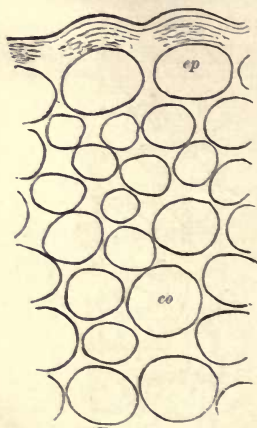
Fig. 54.—Transverse section of collenchyma (co) of the stem of Erhinocystis lobata , wet with water, and the angles greatly swollen. ep, epidermis, with thickened outer wall. \times 700 . From a drawing by J. C. Arthur.
