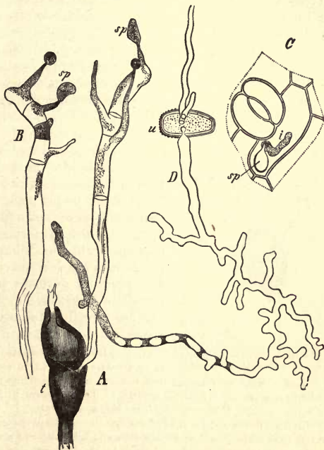
Fig. 217.— Puccinia graminis . A, germinating teleutospore, t , with promycelium forming the sporidia, sp . B, similar promycelium, with sporidia. C, a sporidium, sp , germinating on a piece of the under side of a leaf of the Barberry, the mycelium, i , penetrating the epidermis. D, a germinating uredospore, u , fourteen hours after being placed on the leaf of a grass, forming a branched mycelium. Highly magnified.—After Bè Bary.
