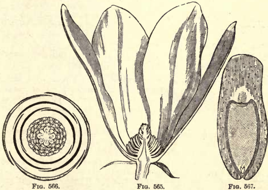
Fig. 565.—Flower cut vertically.
