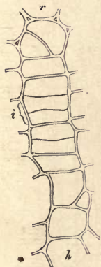
Fig. 325.—The row of cells marked \alpha — \alpha in Fig. 324; r , phloëm; h , xylem; at are seen the fissions of the cambium cells. \times 600 .—After De Bary.
