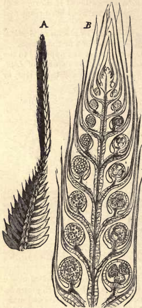
Fig. 278.— A , a fertile branch of Selaginella inaequiloba , with the quadrangular spore-bearing spike at the apex; B , vertical section of the spike, showing the microsporangia containing microspores on the left, and the macrosporangia with macrospores on the right.— A \times 2 ; B \times 15 .—After Sachs
