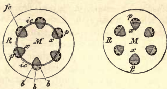
Fig. 323.—Diagrams of dicotyledonous stems as seen in cross-section. R , the cortical, M , the medullary portion of the fundamental system; p , the phloëm; x , the xylem; b, b, b , groups of bast fibres; fc , the fascicular, ic , the interfascicular cambium.—After Sachs.
