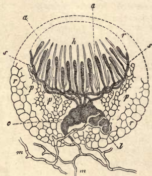
Fig. 197.—Diagrammatic vertical section of the sporocarp of Ascobolus furfuraceus . m, m, mycelium; c, c, carpogonium; l, l, antheridium; s, s, branches bearing the asci, a, a; p, p, pseudo-parenchymatous sterile tissue; r, r, cortical portion of sterile tissue—above it forms the so-called pericarp, which surrounds and encloses the hymenium, h.—After Janczewsky.
