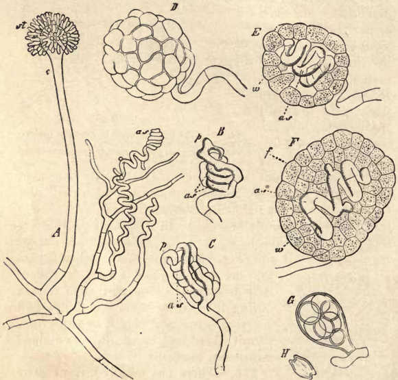
Fig. 191.— Eurotium repens . A , a portion of the mycelium, with erect hyphae, c , bearing at its top a radiating cluster of sterigmata, st , from which the conidia have fallen; as , young carpogonium—below it a younger branch is beginning to coil spirally to form another carpogonium. B , the carpogonium, as , and the antheridium, p . C , the same beginning to be surrounded by the enveloping branches which grow out from its base. D , sporocarp. E, F , sections of ripe sporocarps; w , outer wall; f , inner cells of sterile tissue; as , developing carpogonium, giving rise to branches from which asci are produced. G , an ascus containing eight ascospores. H , ripe ascospore. Highly magnified.—After De Bary.
