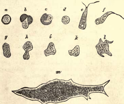
Fig. 141.— Fuligo varians ( Æthallium septicum of Fr.). a spore; b, c , spore-case rupturing and permitting the protoplasmic contents to escape; d , rounded mass of naked protoplasm escaped from the spore-case; e, f , ciliated swarm-spore or zoospore stage; g, h, i, k, l , amoeba stage; m , young plasmodium.—After Prantl.
