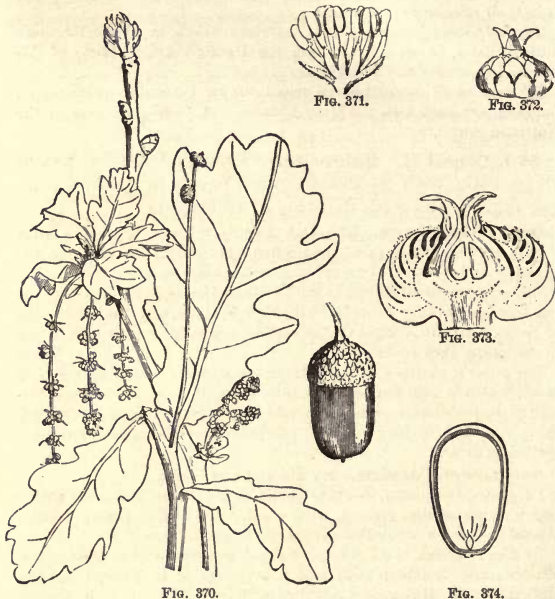
FIGS. 370-74.—ILLUSTRATIONS OF QUERCUS ROBUR.
