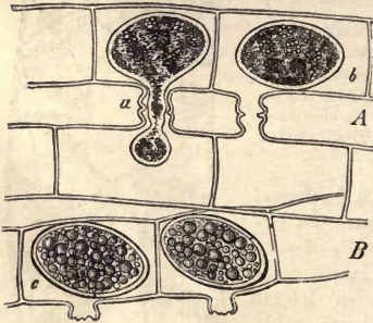
Fig. 37.—Filaments of Sproggyra longata ; in A , at a the protoplasm is passing from the lower cell to the upper; at b the union of the two protoplasmic masses is completed; in B the protoplasmic masses have secreted thick walls, thus completing the formation of the new cells. \times 550 .—After Sachs.
