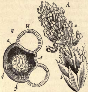
Fig. 281.—A, a male flower of Abies pectinata ; b, bracts; a, stamens. B, pollen grain; e, extine, with its large vesicular protrusions, bl; i, intine; y, cell in the interior of the pollen grain developing the pollen tube; g, basal cell attaching y to the wall of the grain. \times 300 —A after Sachs; B after Schacht.
