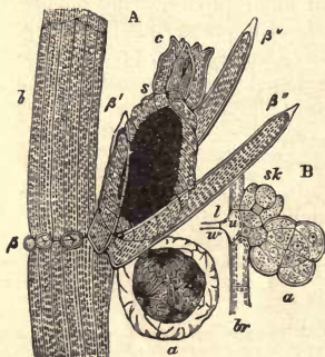
Fig. 228.—Reproductive organs of Chara fragilis . A , a central portion of a leaf, b , with an antheridium, a , and a carpogonium, c , surrounded by the spirally twisted enveloping cells; c , crown of five cells at apex; \beta , sterile lateral leaflets; \beta' , large lateral leaflet near the fruit; \beta'' , bracteoles springing from the basal node of the reproductive organs. B , a young antheridium, a , and a young carpogonium, sk ; w , nodal cell of leaf; u , intermediate cell between w and the basal node cell of the antheridium; l , cavity of the internode of the leaf; br , cortical cells of the leaf. A \times about 33; B \times 240.—After Sachs.
