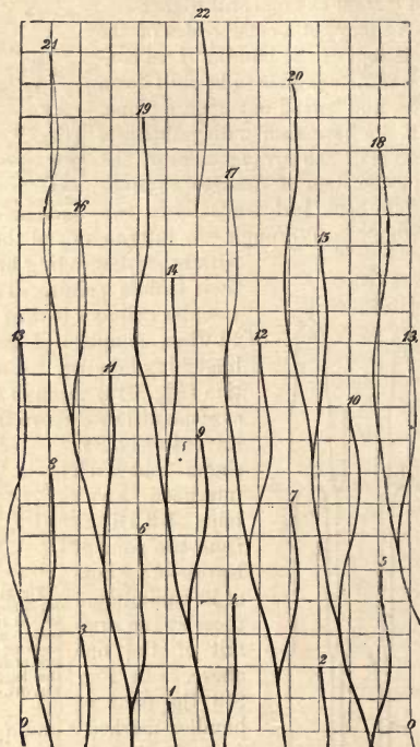
Fig. 319.—Diagram showing the arrangement of the fibro-vascular bundles in 22 internodes of the stem of Iberis anara .—After Nägeli.
