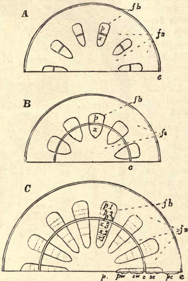
Fig. 301.—Diagrammatic cross-sections of the stem of Gymnosperms. A , young stem with the fibro-vascular bundles, fb , widely separated; p , the phloem; x , the xylem; fs , tissues of the fundamental system; e , epidermis. B , a similar section of an older stem, the cambium layer, c , extended through the fundamental system from bundle to bundle. C , section of a three-year-old stem, showing the manner of increase in the xylem and phloem; pc , primary cortex (phloem); sc , secondary cortex (phloem); c , cambium layer; sw , secondary wood (xylem); pw , primary wood (xylem); p , plth; p1 , p2 , p3 , x1 , x2 , x3 , corresponding phloem and xylem portions of each year's growth of the bundle.
