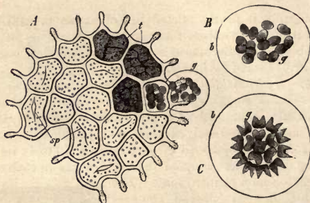
Fig. 151.—A, a colony of cells constituting a so-called individual of Pediastrum granulosum ; t , cells with their contents remaining; the white cells are empty, their contents having escaped by the slits sp ; g , contents of a cell (macrozoogonidia) escaping. B, macrozoogonidia g , in the motile state, enclosed in the membrane b . C, the macrozoogonidia arranging themselves in a colony, still enclosed by the membrane b . \times 400 .—After Braun.
