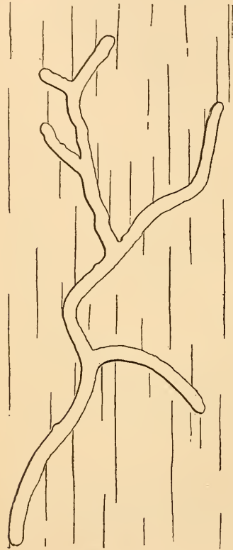
FIG. 63.— Dendroctonus approximatus : Single egg gallery. (Original.)
