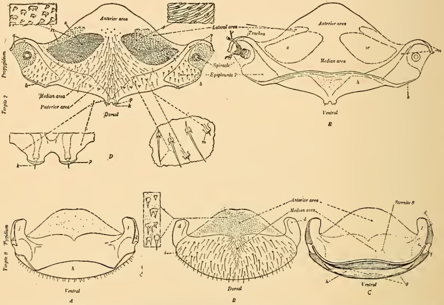
FIG. 23.— Dendroctonus valens : Male, abdominal tergites 7 and 8. A , Tergite 8 (pygidium), ventral; B , same, dorsal; C , same, ventral, showing position of sternite 8; D , tergite 7 (propygidium), dorsal; E , same, ventral; a , anterior arm of epipleurite 7; b , posterior arm of epipleurite 7; c , membranous lobe; d , epipleural process; e , hypopleural arm of sternite 8; f , pleural opening; g , anal space; h , ventral fold; i , rudimentary spiracle 8; j , epipleural disk; k , apical spine; l , stridulating process; m , sensory bristles; n , enlarged section of lateral area; o , enlarged section of membranous lobe; p , stridulating scraper. (Original.)
