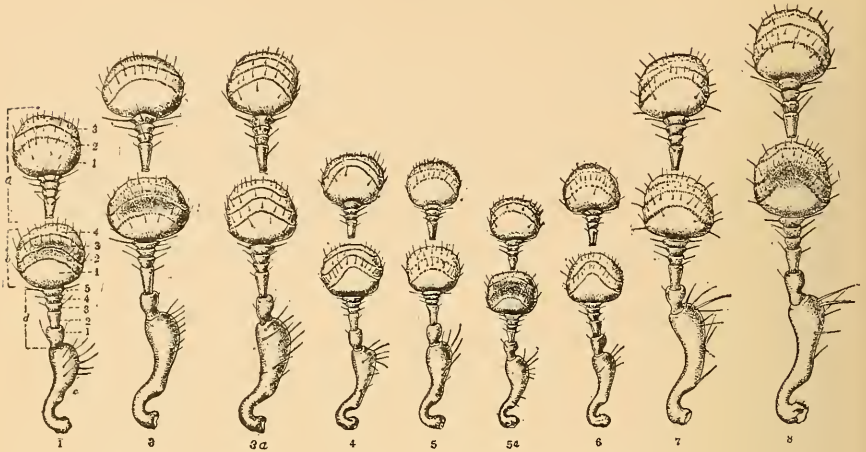
FIG. 11.— Dendroctonus : Antennæ. 1, brevicornis ; 3, converifrons ♀; 3a, converifrons ♂; 4, frontalis ♂; 5, arizonicus ♂; 5a, arizonicus ♀; 6, mexicanus ; 7, parallelocollis ; 8, approximatus ♀. (Original.) 1—a, posterior face of club when antenna is extended at right angles to head, joints 1, 2, 3; b, anterior face, joints 1, 2, 3, 4; d, funiculus, joints 1, 2, 3, 4, 5; c, scape.
