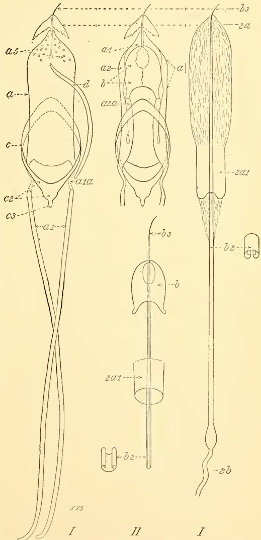
FIG. 103.— Ips cmarginatus : Chitinous elements of male reproductive organs. I, ventral aspect; II, dorsal aspect. See terminology, Division 1, pp. 192-193. (Original.)
