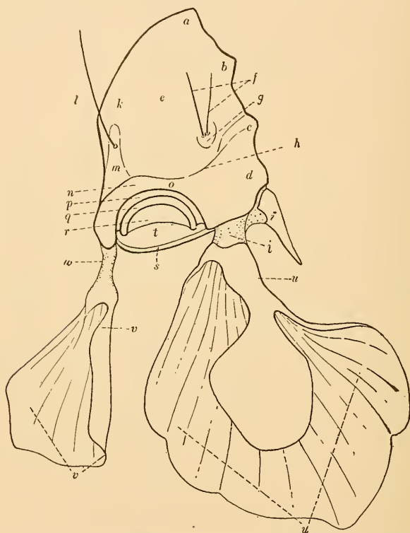
FIG. 14.— Dendroctonus valens : Mandible. a , Apical tooth; b , subapical tooth; c , median tooth; d , molar tooth; e , dorsal area; f , dorsal bristles or setæ; g , dorsal impression; h , transverse ridge; i , pharyngeal process; j , retractor tendon; k , lateral area; l , lateral bristle; m , lateral impression; n , anterior condyle; o , basal ridge; p , median fossa; q , median condyle; r , posterior fossa; s , condyle of ventral articulation; t , basal foramen; u , retractor disk; v , extensor disk; w , extensor tendon. (Original.)
