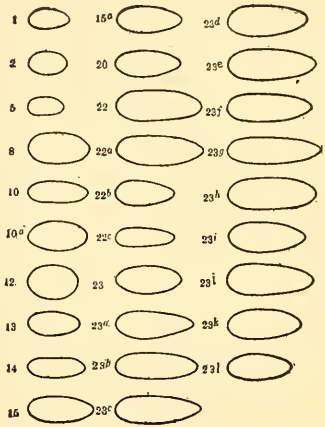
FIG. 15.— Dendroctonus : Eyes. 1, brevicornis ; 2, barberi ; 5, arizonicus ; 8, approximatus ; 10, 10a, ponderosæ ; 12, simplex ; 13, pseudotsugæ ; 14, piceaperda ; 15, 15a, engelmanni ; 20, punctatus ; 22, 22a, b, c, terebrans ; 23, 23a, b, c, d, e, f, g, h, i, j, k, l, valens . (Original.)
