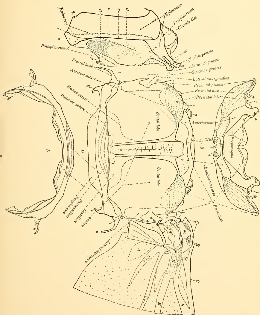
FIG. 20.— Dendroctonus valens : Metatergum and metapleurum. B , Anterior aspect of prephragma and postscutum; D , metatergum and metapleurum; E , posterior aspect of postphragma and postscutellum; a , lateral arm of prephragma; b , dorsal band; c , scapular plate; d , subscapular plate; e , flexor plate; f , radial plate; g , medial plate; h , lateral arm of postphragma; i-i , metatergal costæ; j , anterior disk; k , scutellar groove; l , posterior ridge; o , exposed triangular plate of postepimeron; p , pleural hinge; pc , pleural clavicle; q , posterior ventral angle of episternum; r , anterior ventral angle of episternum; s , pleural suture; t , postsutellar process; u , clavicle condyle; v , coracoid condyle; w , attachment and articulation of scapular plate; x , dorsal area of postscutellum; y , pleural disk; z , elevated acute margin; z1 , membranous area; z2 , villous area. Wing veins: C , costa; Sc , subcosta; R , radius; M , media; Cu 1 , cubitus 1; Cu 2 , cubitus 2; A , anai. (Original.)
