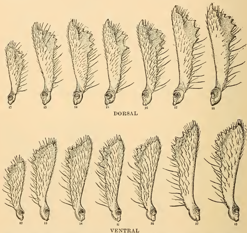
FIG. 28.— Dendroctonus : Left tibiae, dorsal and ventral aspects. 12, simplex ; 13, pseudotsugæ ; 14, piceaperda ; 15, engelmanni ; 16, borealis ; 17, obesus ; 18, rufipennis . (Original.)
