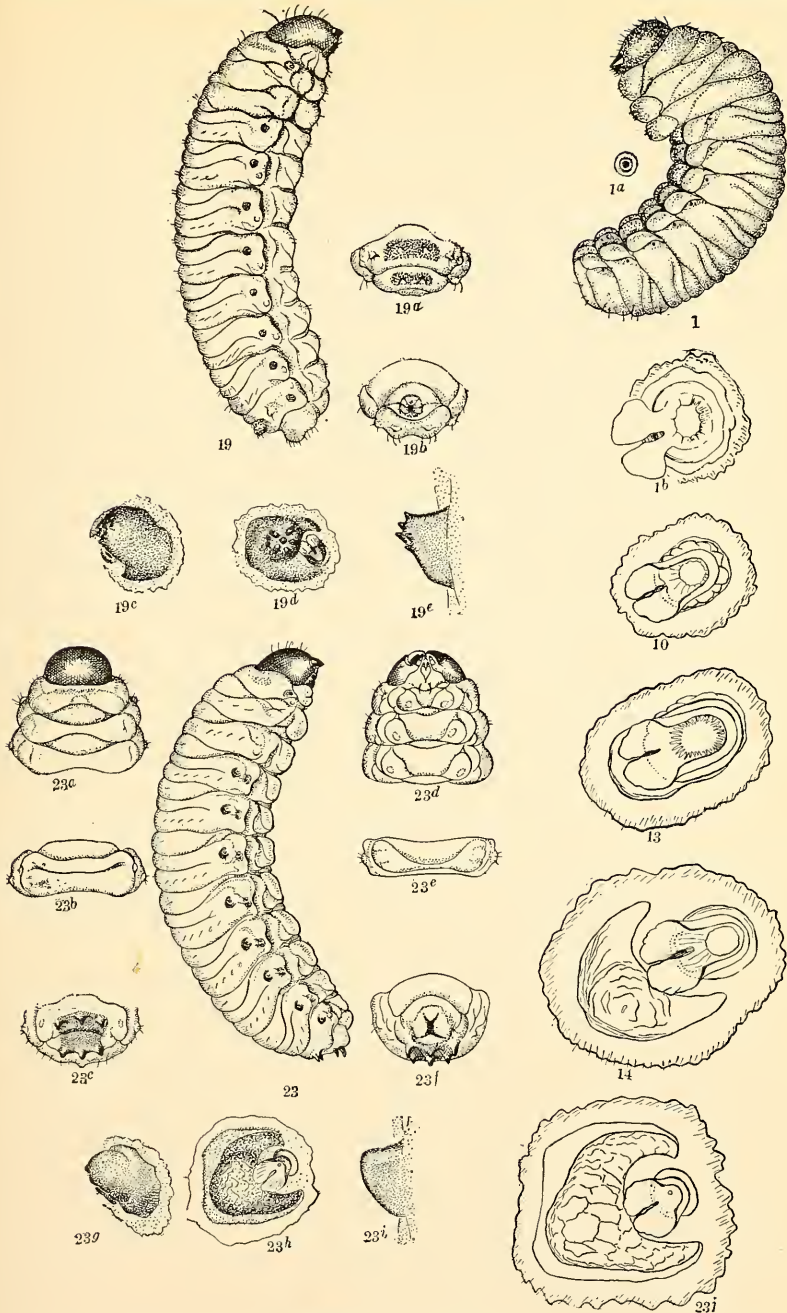
Fig. 1.— D. brevicornis ; 1a, spiracle, enlarged; 1b, spiracle, greatly enlarged, showing simple bifid processes. Fig. 10.— D. ponderosa , spiracle, greatly enlarged. Fig. 13.— D. pseudotsugae , spiracle, greatly enlarged. Fig. 14.— D. piceaperda , spiracle, greatly enlarged. Fig. 19.— D. murrayanae ; 19a, dorsal aspect of abdominal segments 8 and 9, showing plates; 19b, anal aspect; 19c, 19d, and 19e, different aspects of spiracular tubercle, much enlarged. Fig. 23.— D. valens ; 23a, dorsal aspect of thoracic segments; 23b, dorsal aspect of abdominal segments; 23c, dorsal aspect of abdominal segments 8 and 9, showing armed plates; 23d, ventral aspect of thoracic segments; 23e, ventral aspect of abdominal segment; 23f, anal aspect of abdominal segments 8, 9, and 10; 23g, 23h, 23i, different aspects of spiracular tubercles, moderately enlarged; 23j, spiracle and spiracular tubercle, greatly enlarged. (Original.)
