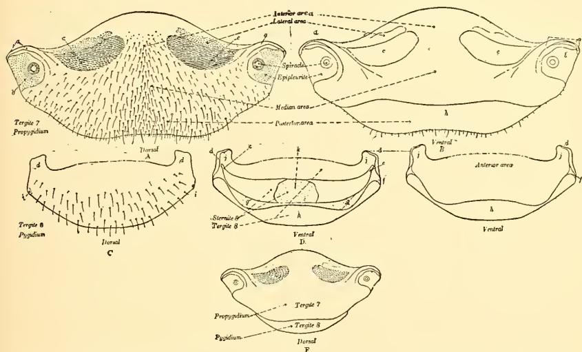
FIG. 24.— Dendroctonus vulens : Female, abdominal tergites 7 and 8. a , Anterior arm of epipleurite 7; b , membranous area surrounding spiracle; c , membranous lobe; d , epipleural process; e , hypopleural process of sternite 8; f , pleural opening; g , anal space; h , ventral fold; i , rudimentary spiracle; j , epipleural disk; k , median membranous connection of the lateral sections of sternite 8. (Original.)
