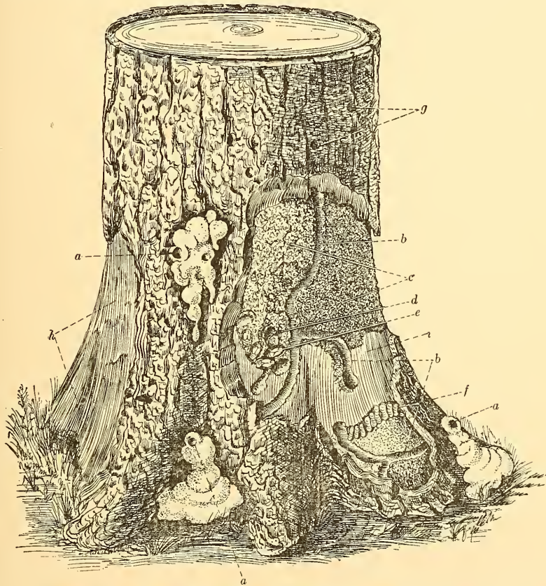
FIG. 92.— Dendroctonus valens : Work in bark at base of stump. a , Entrance and pitch tube; b , egg gallery; c , boring dust and resin; d , pupal cell; e , pupa; f , larvæ at work feeding on inner living bark; g , exit burrows; h , resulting old scar or basal wound, often referred to as basal fire wound; i , inner bark with outer corky bark removed. (Original.)
