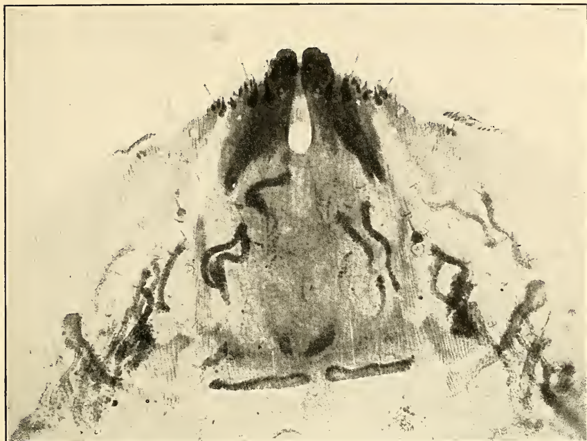
FIG. 1.—ASPIDIOTUS (DIASPIDIOTUS) AFRICANUS.
