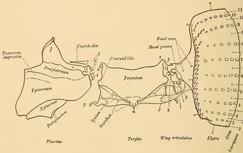
FIG. 19.— Dendroctonus valens : Mesotergum and mesopleurum. a , Lateral arm of prephragma and prescutum; b , wing root or connecting membrane; c , basal margin of elytra; d , radial plate; e , flexor plate; f , median plate; g , scapular plate; h , subscapular plate; i , sutural or anal margin; j , preepisternal process; k , clavicle condyle; l , coracoidal condyle; m , scutellum; n , lateral margin of elytra; o , arm of preepisternal process; striae 2-10; interspaces 2-11; p , lateral arm of postphragma; q , pleural clavicle. (Original.)
