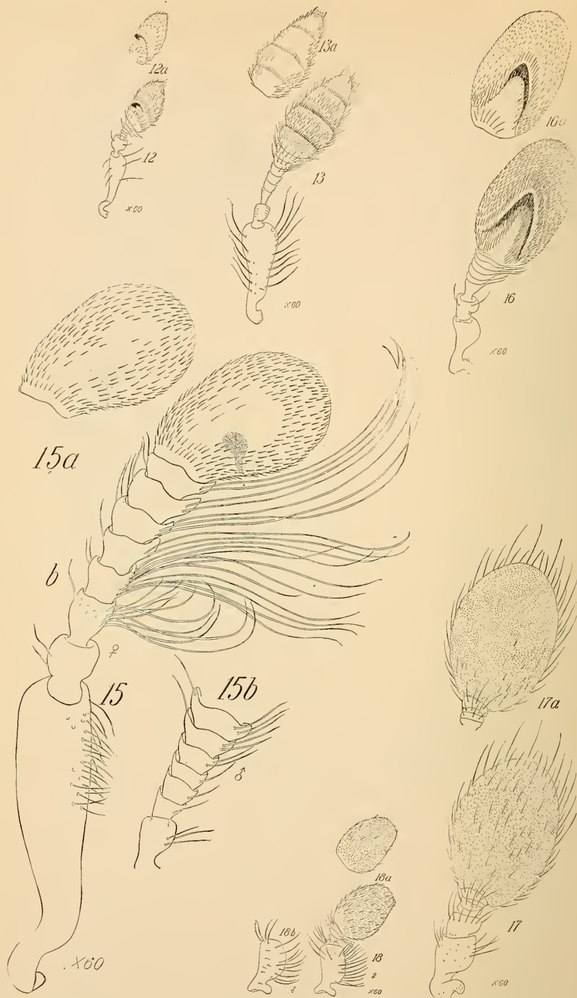
Fig. 12.— Hexacolus sp. (Hexacoliniæ), anterior aspect of left antenna. Fig. 12a.—Posterior aspect of left antenna of same. Fig. 13.— Bothrosternus sculpturatus (Bothrosterninæ), anterior aspect of left antenna. Fig. 13a.—Posterior aspect of left antenna of same. Fig. 15.— Campocerus æneipennis (Campocerinæ), anterior aspect of left antenna of female. Fig. 15a.—Club of female of same. Fig. 15b.—Scape of male of same. Fig. 16.— Scolytus scolytus (Scolytinæ), anterior aspect of left antenna. Fig. 16a.—Posterior aspect of left antenna of same. Fig. 17.— Scolytoplatypus sp. (Scolytoplatypodinæ), anterior aspect of left antenna. Fig. 17a.—Posterior aspect of left antenna of same. Fig. 18.— Platypus cylindrus (Platypodinæ), anterior aspect of left antenna of female. Fig. 18a.—Posterior aspect of left antenna of same. Fig. 18b.—Male scape of same. (Original.)
