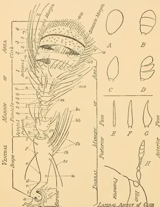
FIG. 96.—The antenna in scolytoid beetles: Diagram and terminology. Scrobe: a , Fossa. Scape: b , Condyle; c , basal section or neck; d , elbow; e , median section; f , apical section; ga , dorsal fringe; g , apical fossa; ga , apical margin. Funicle: h , Base or condyle; i , basal section; j , median section; k , apical section; ka , apical angle; kb , dorsal lobe; l , ventral angles of joints; m , dorsal angles; ma , funicular fringe or dorsal bristles; n , apical joint. Club: o , Basal annulation; p , apical or sutural annulation of joint 1; q , ventral septum or single septum; r , dorsal and ventral septa or double septa; s , chitinous suture; t , ventral fringe; ta , ventral bristle; tb , procumbent bristle; tc , recumbent bristle; u , setaceous annulation or sutural annulation; v , sensitive pores; w , sensitive and setal granules; wa , sensitive area; wb , chitinous area. Club: A , solid; B , annulated; C , conical; D , separated joints or sublamellate; E , compressed; F , thickened at base; G , obliquely truncate; H , antenna extending at right angles to the head. (Original.)
