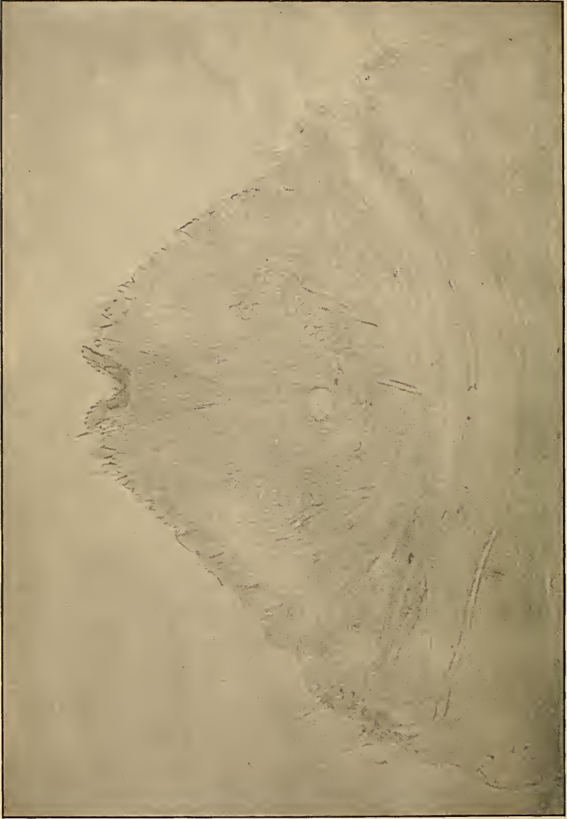
ANAL PLATE OF FIORINIA FIORINÆ VAR. MINOR. MAGNIFIED 515 DIAMETERS. (ORIGINAL.)
