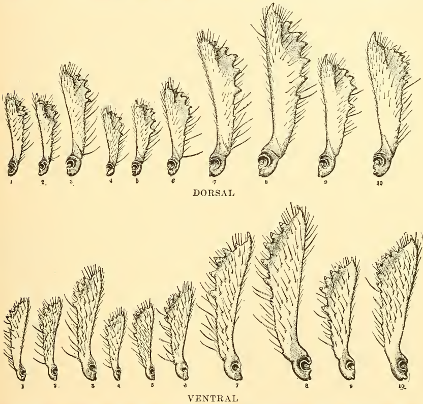
FIG. 27.— Dendroctonus : Left tibiæ, dorsal and ventral aspects. 1, brevicomis ; 2, barberi ; 3, convexifrons , 4, frontalis ; 5, arizonicus ; 6, mexicanus ; 7, parallelcollis ; 8, approximatus ; 9, monticolæ ; 10, ponderosæ . (Original.)
