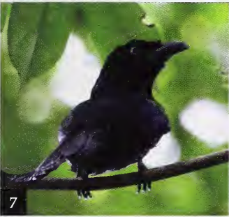
Figure 7. Hair-crested Drongo Dicrurus hottentottus banggaiensis , Peleng at c.600 m, March 2009 (F. Verbelen). Note the greyish irides.
