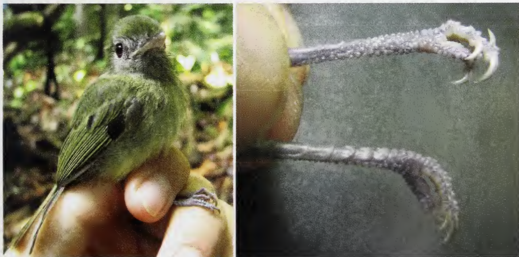
Figure 1. Boat-billed Tody-Tyrant Hemitriccus josephinae (and its noduled tarsi), near Manaus, Brazil (E. I. Johnson)
