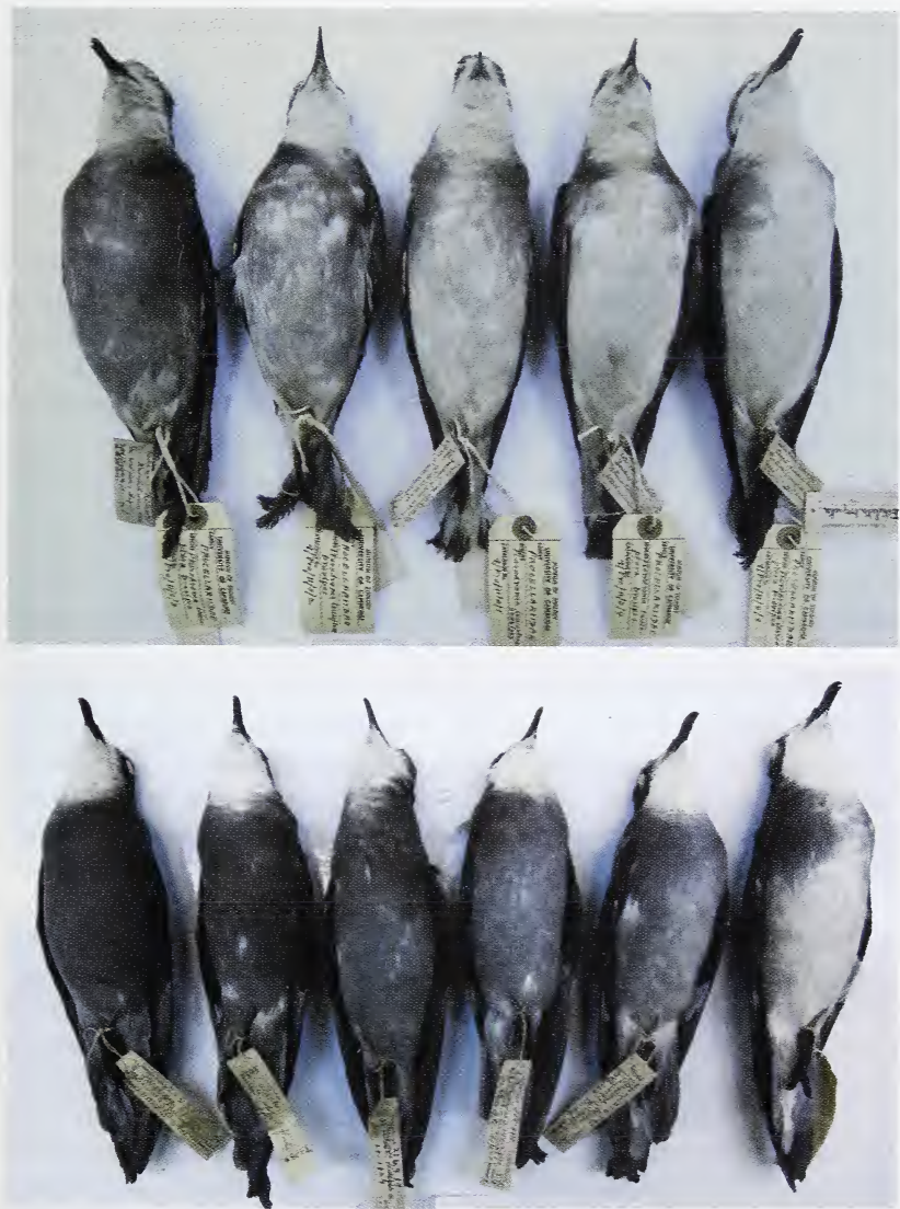
Figure 1 (top). Five specimens of Collared Petrel Pterodroma brevipes collected in Fiji, in the interior of Viti Levu (University Museum of Zoology, Cambridge, UK), showing the basic colour variation in the species. Plumage types are adopted from Watling (1986), which were used to score specimens and live birds at sea. From right to left: ‘pure white’—the two right-hand specimens (this category includes completely clean white-bellied birds as well as those with a few very indistinct dark feather tips); ‘grey peppering’—the middle specimen, with variable dark mottling and dappling, giving the underparts a blotchy appearance, but with a predominantly white belly; ‘smoky’—fourth from right, with variable grey wash, but ground colour still pale and contrasts with breast-band, and many birds appear faintly blotched below (much individual variation between this, the previous and next categories); ‘dark grey’—the left-hand specimen, with rather medium / dark and uniform grey pigments, and the dark breast-band is not obvious but still detectable in most. No ‘extreme dark grey’ type was found in collections other than in P. b. magnificens (Fig. 2). The percentage of each colour type is given in Table 2 (Hadoram Shirihai, © Tubenoses Project)
