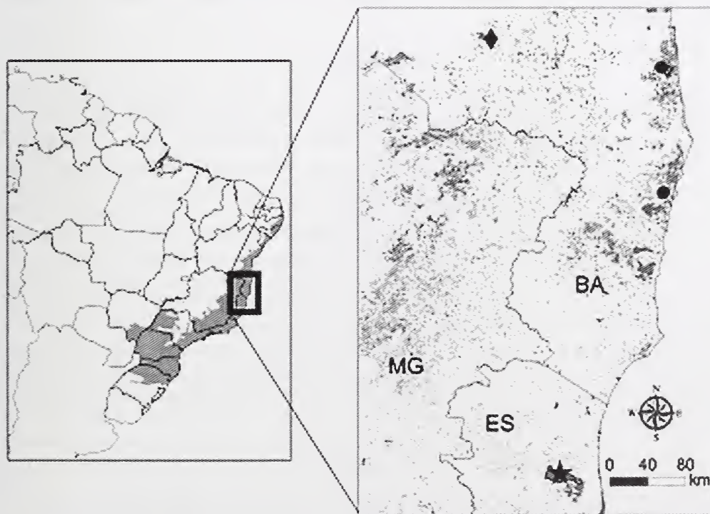
Figure 1. Map showing the Atlantic Forest biome (shaded; left) and Brazilian states of Minas Gerais (MG), Bahia (BA) and Espírito Santo (ES), with recent and historical records of White-winged Potoo Nyctibius leucopterus in the Atlantic Forest (right). The diamond marks the type locality at Vitória da Conquista, Bahia, circles other recent records and the star our record at Sooretama Biological Reserve, Espírito Santo.
