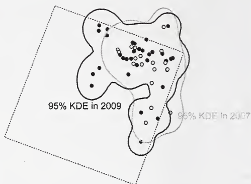
Figure 4. Home range estimates for H. josephinae based on 95% kernel density estimates (KDE) using spot-mapped points in a 10-ha fragment (dotted black line indicating the border) in 2007 (grey) and 2009 (black) near Manaus, Brazil.
