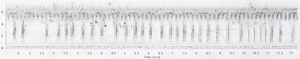
Figure 12. Sonogram of the distinctive alarm vocalisation of Gray's Grasshopper Warbler Locustella fasciolata recorded at 800 m on Peleng. The recording constitutes a rapid series of call doublets ( terreck-terreck, terreck terreck-terreck . . .). Dark smudging at 0.6 kHz is background noise of insects. X-axis = time (0.5 seconds per tick), y-axis = frequency (2 kHz per tick). Recording by F. Verbelen.
