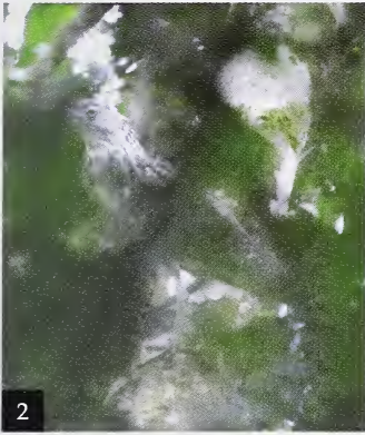
Figure 2. Malayan Night Heron Gorsachius melanolophus kutteri , western Peleng at c.850 m, 28 March 2009 (F. Verbelen)
